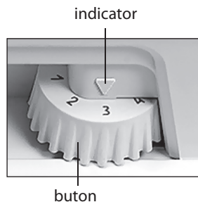
Figura 4 – Buton
